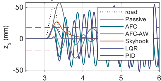
Bump 50 mm x 2.5 m at 20 km/h
