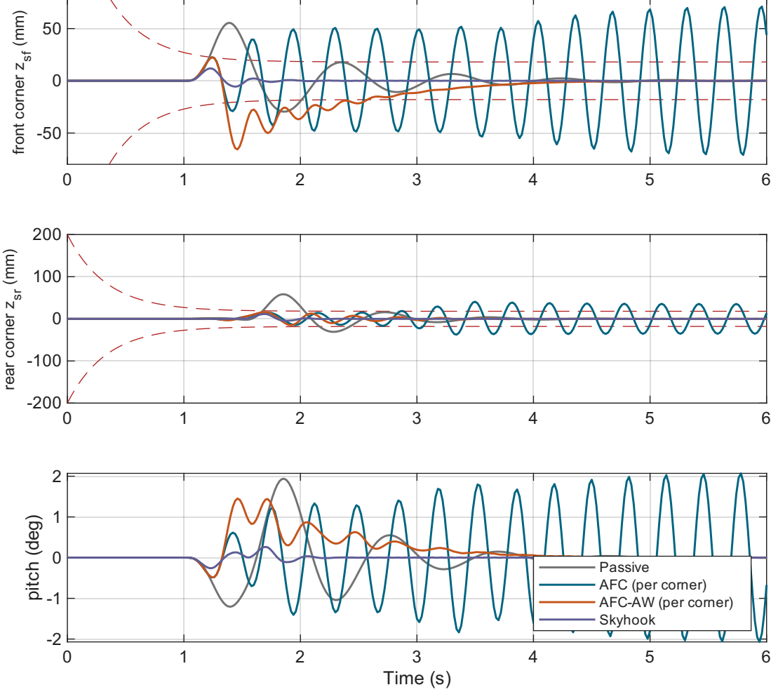
Half car ( I = 1100 \text{ kg m}^2 , a = 1.2 \text{ m} , b = 1.4 \text{ m} ), road: bump
