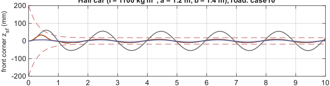
Half car ( I = 1100 \text{ kg m}^2 , a = 1.2 \text{ m} , b = 1.4 \text{ m} ), road: case10
