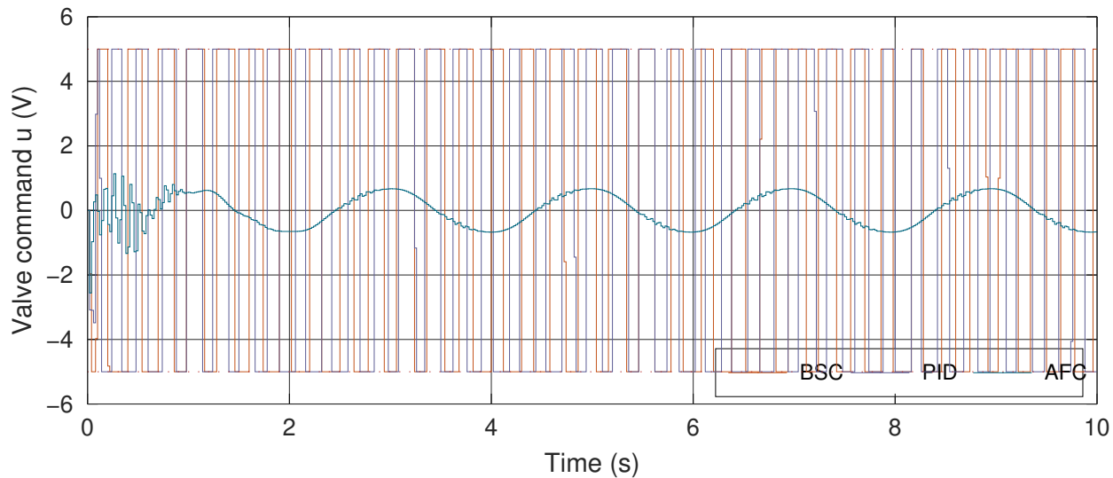
Applied control voltage (paper Fig. 10 analogue)
