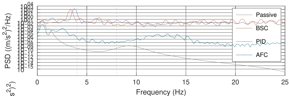
Acceleration spectrum; dotted lines mark the paper's 4–8 Hz band
