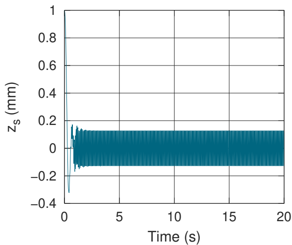
No road: bounded oscillation
