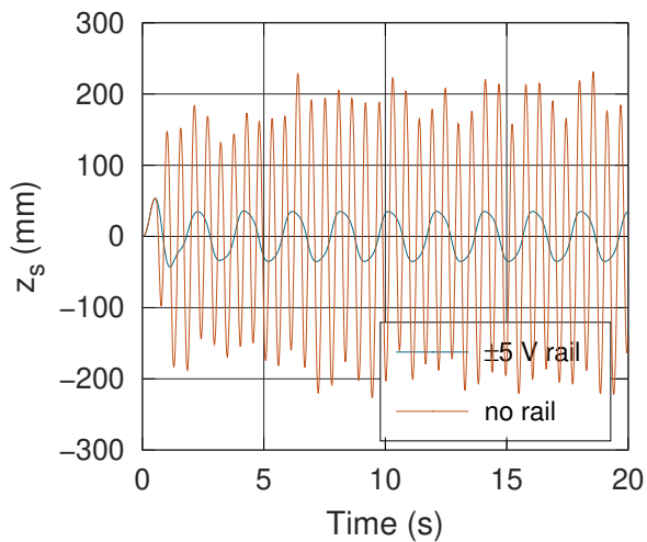
v1: no rail is worse
