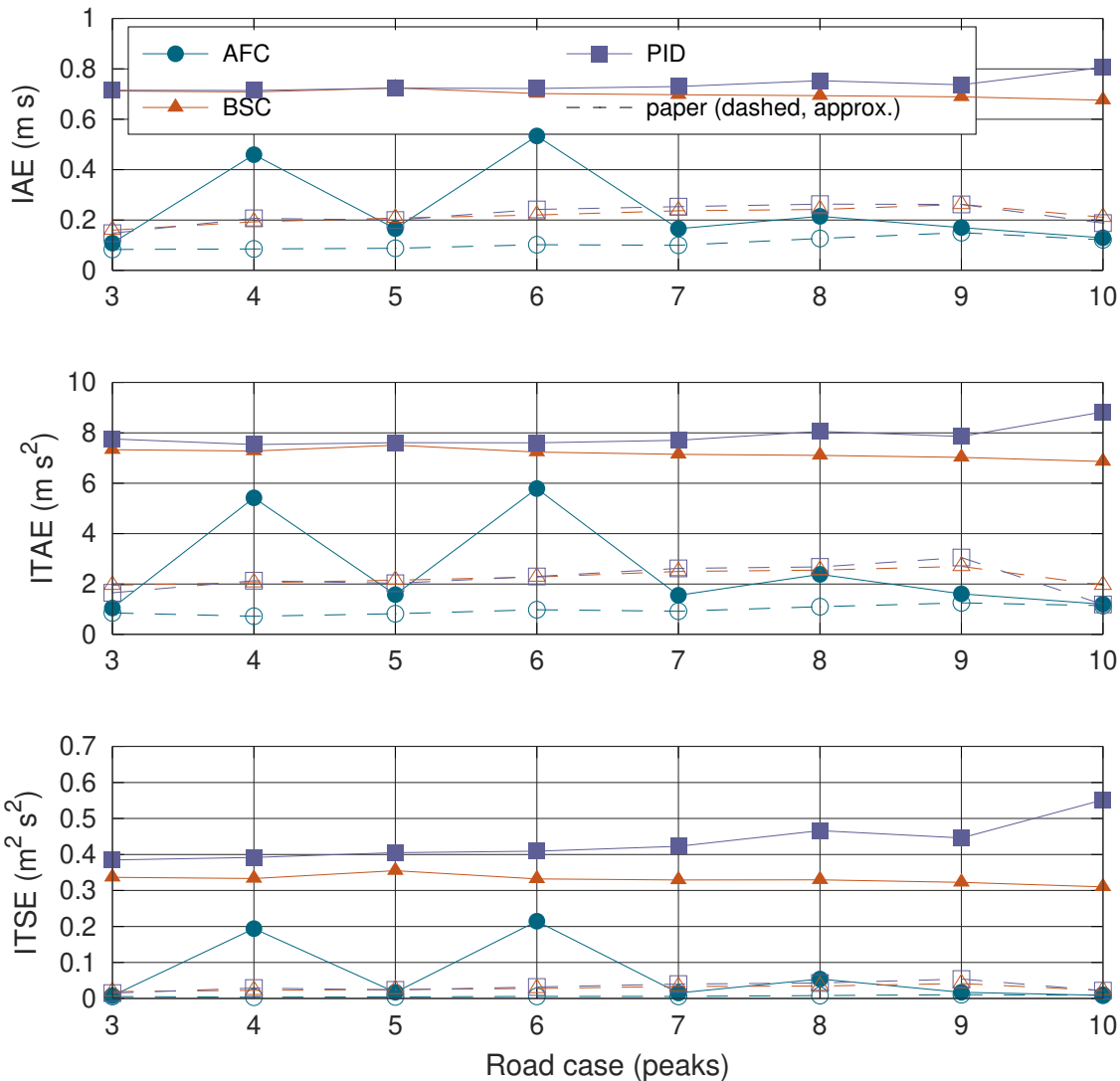
Road sweep: simulation (solid) vs paper Fig. 12 (dashed)
