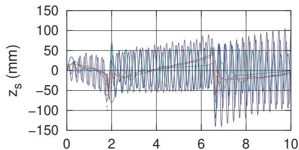
ISO 8608 class C at 54 km/h
