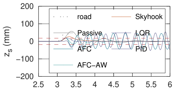
Bump 50 mm x 2.5 m at 20 km/h
