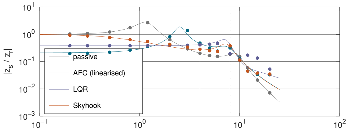
Road-to-body transmissibility: lines = continuous linearised, dots = sampled nonlinear
