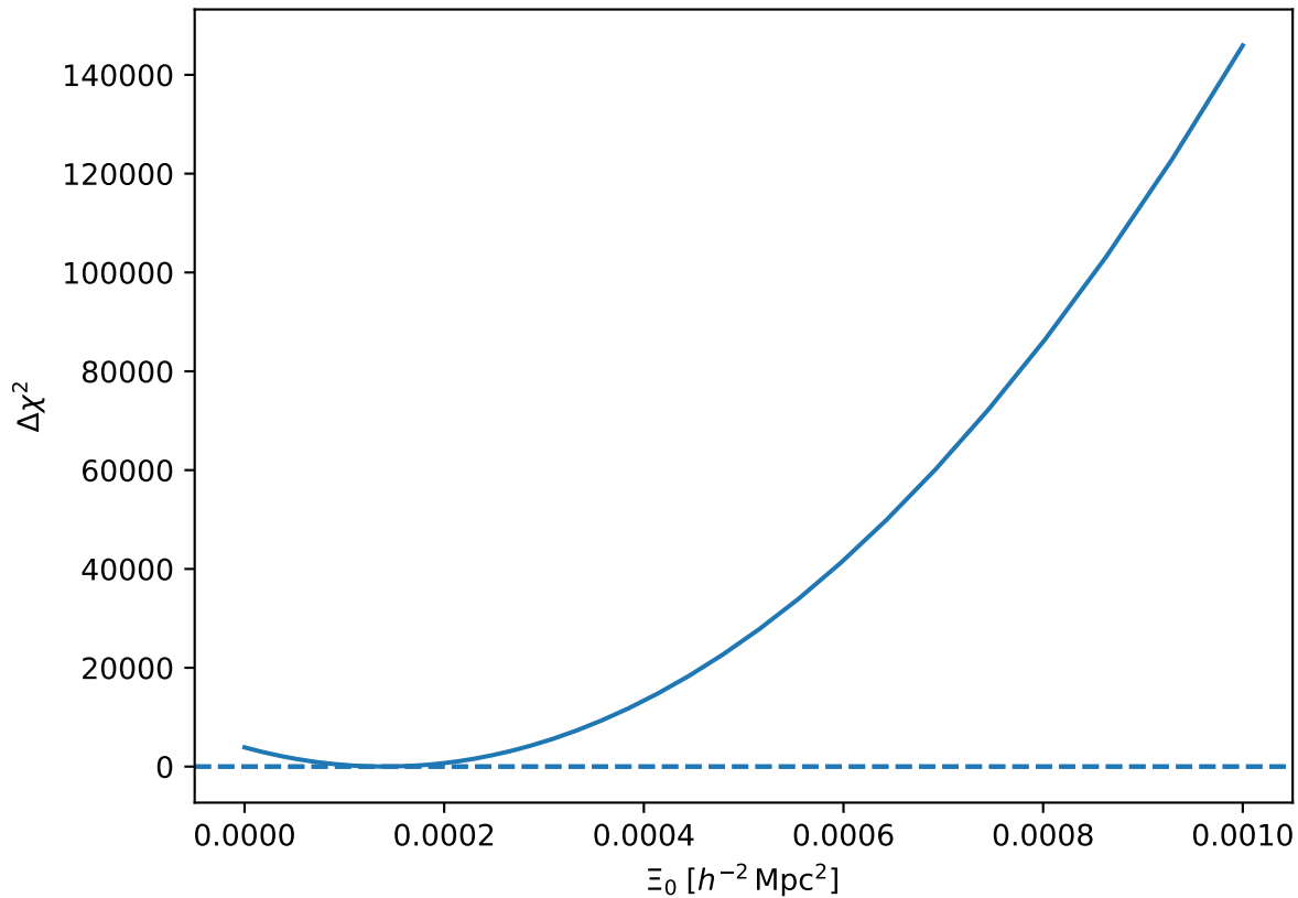
DESI Ly \alpha 1D Constraint on DLSFH Transport
