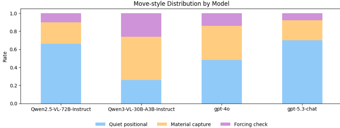
Figure 5: Move-style distribution for successful move-selection benchmark rows.
