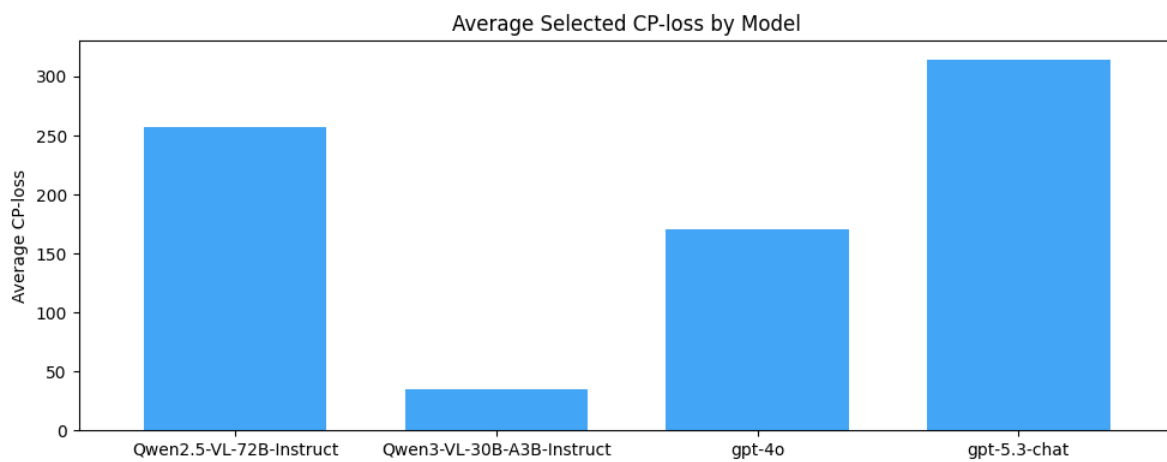
Figure 4: Average selected centipawn loss by model in the move-selection benchmark.
