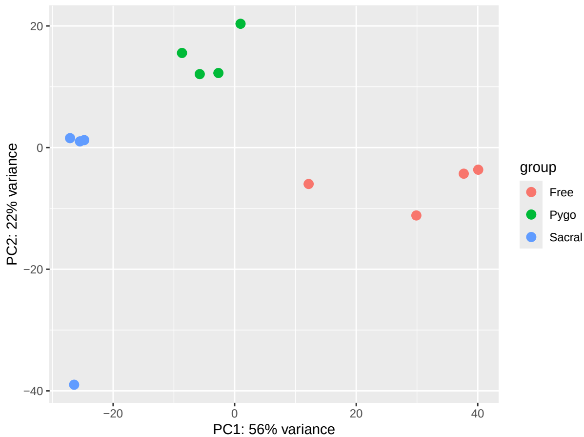
PCA – variance–stabilised counts
