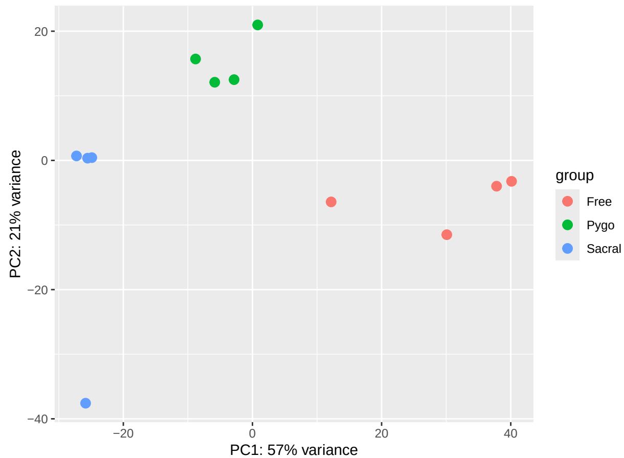
PCA – variance–stabilized counts
