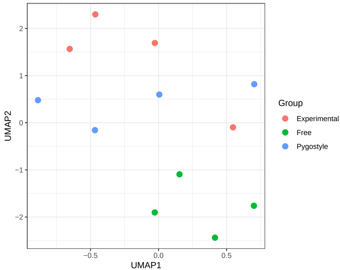
UMAP of samples (ssGSEA scores)
