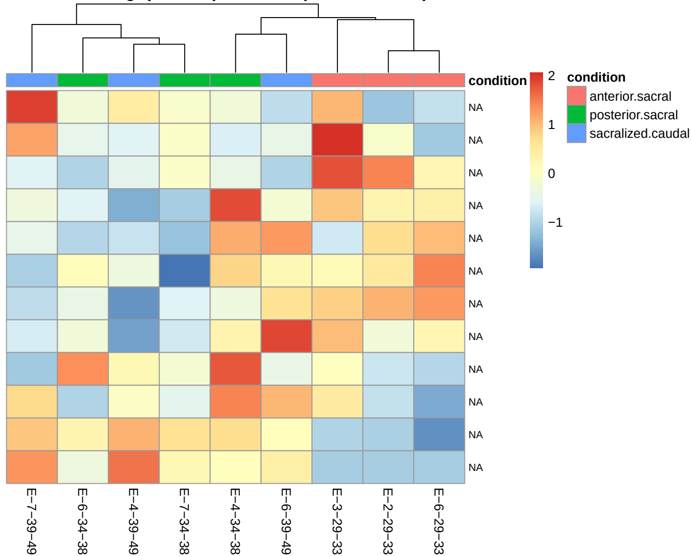
HOXA - log2(norm+1) z-scored (ordered 1->13)
