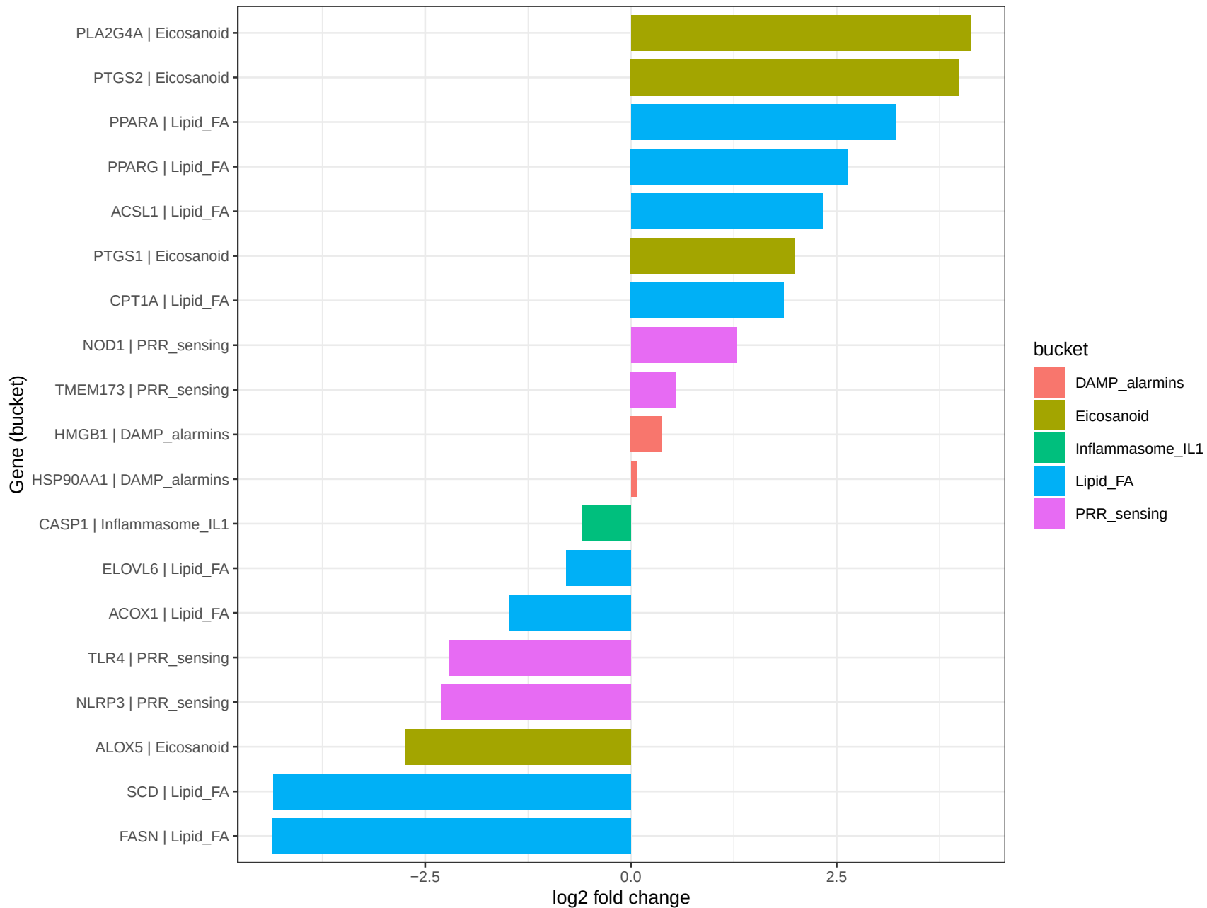
DAMP/FA panel genes in input
