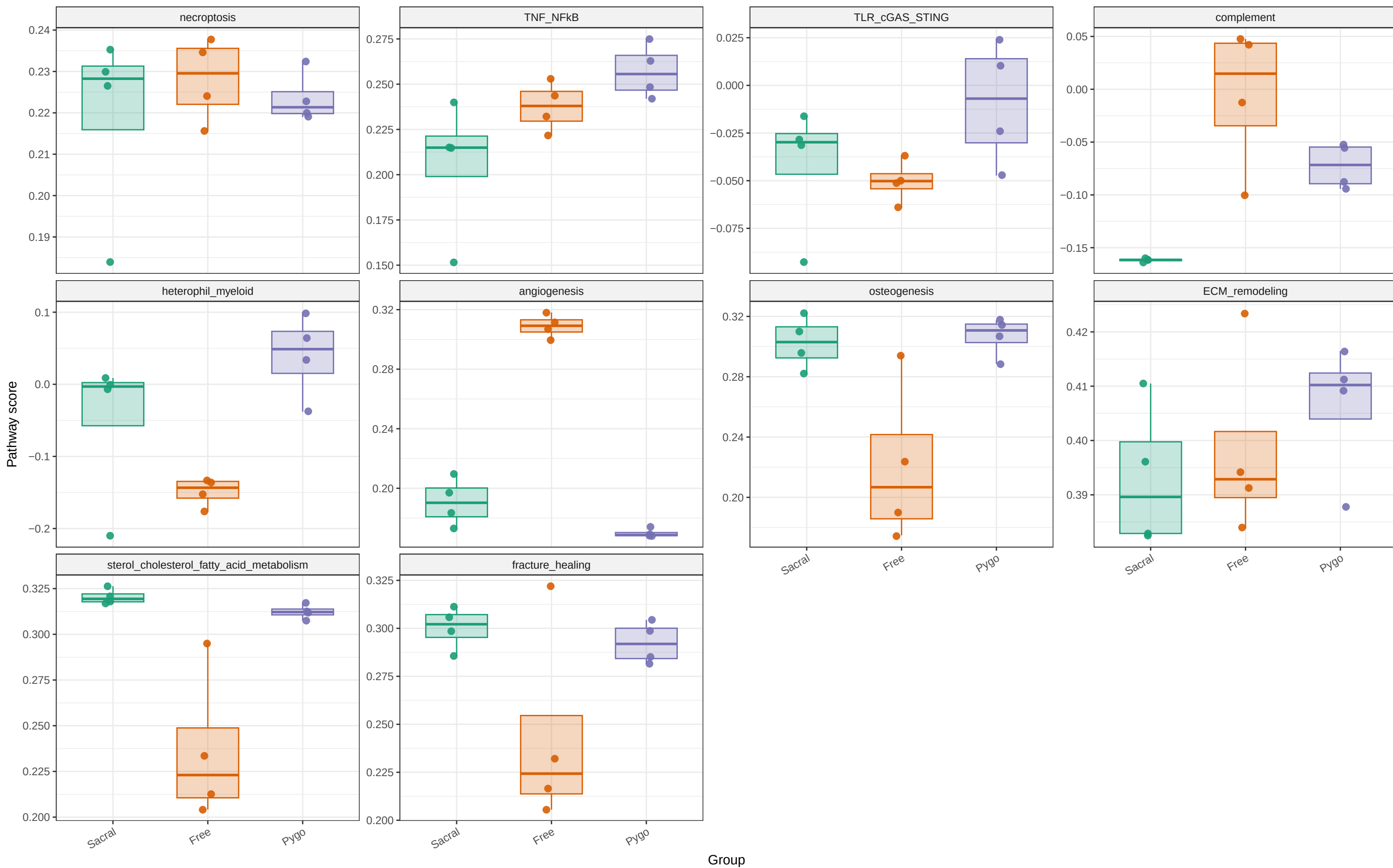
SINGSCORE pathway scores by group
