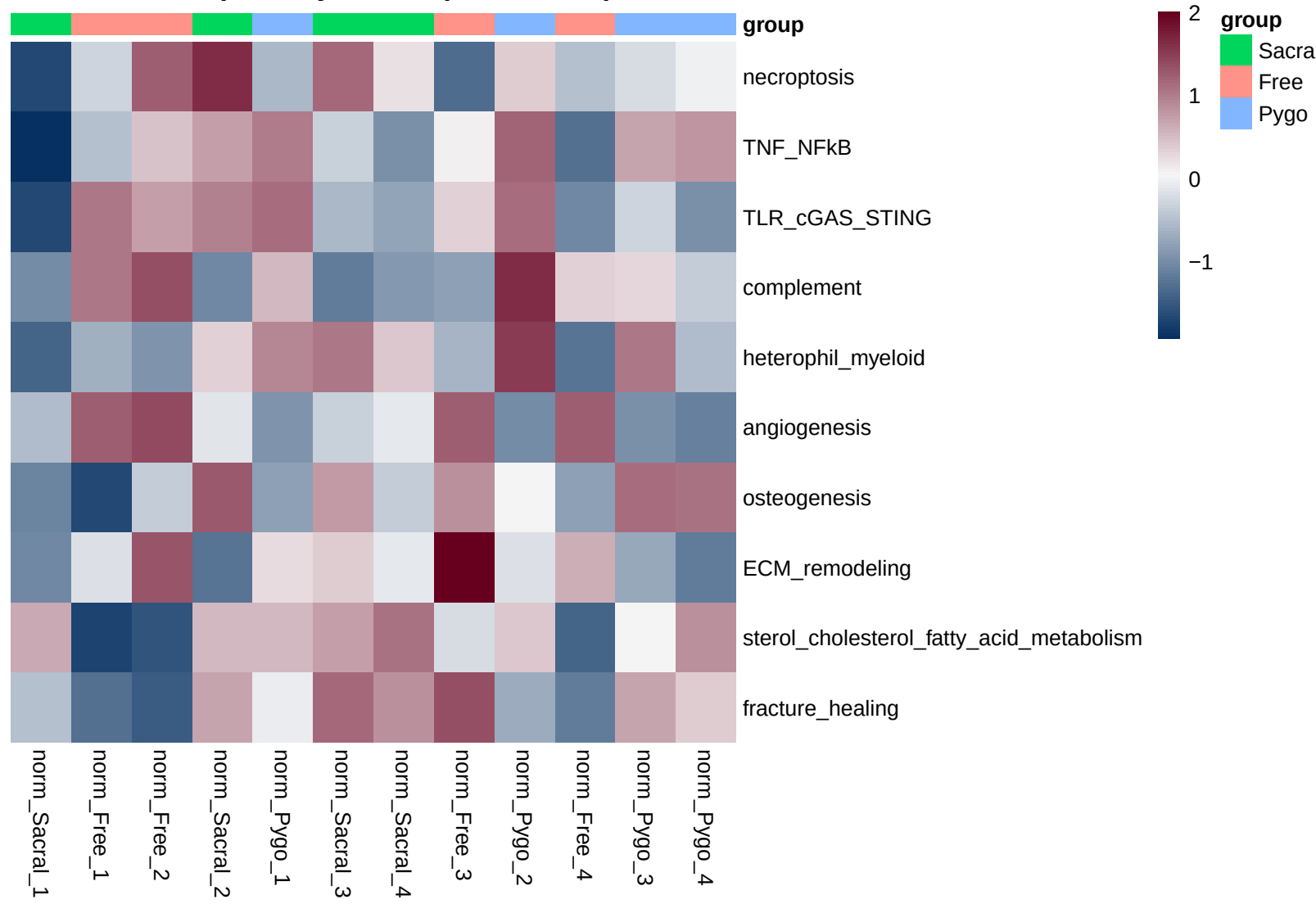
GSVA pathway scores (row-scaled)
