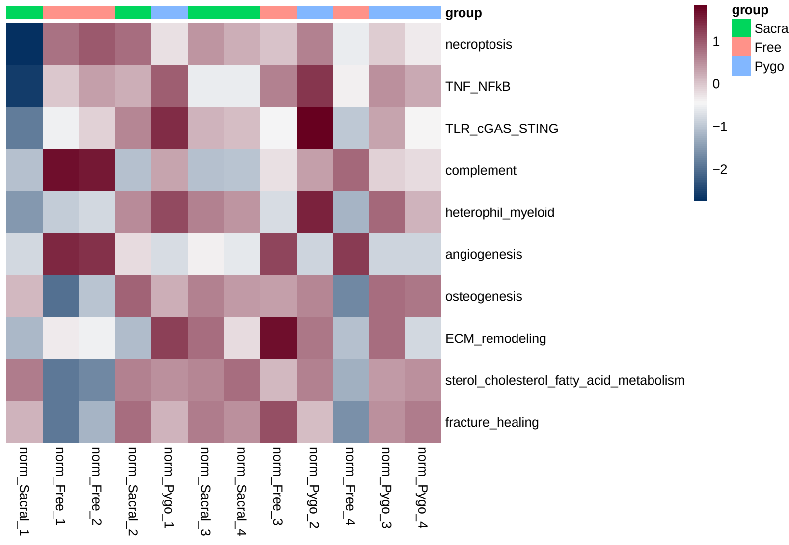
SINGSCORE pathway scores (row-scaled)
