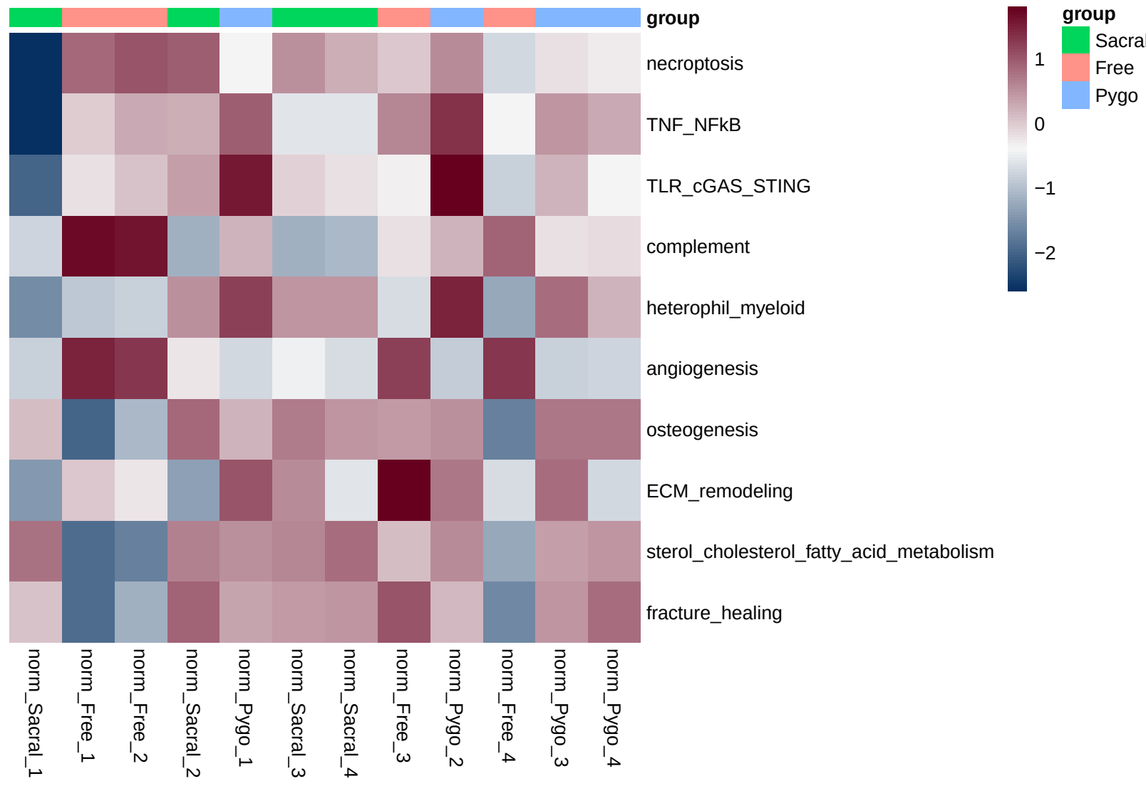
SSGSEA pathway scores (row-scaled)
