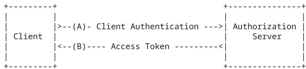
Figure 6: Client Credentials Flow
