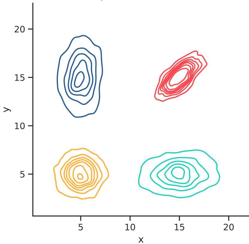
Joint distribution
