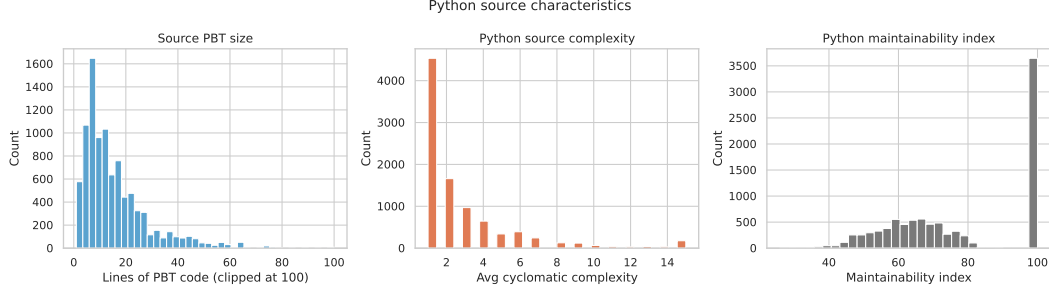
Figure 2: Code-quality metrics for the 11,039 deduplicated PBTs, computed by Radon [1]. Left : lines of code. Center : cyclomatic complexity—the number of linearly independent execution paths through the function, i.e. one plus the number of binary branch points [40]; higher values indicate more complex control flow. Right : maintainability index—a 0–100 composite of Halstead volume [20], cyclomatic complexity, and source lines, where higher is more maintainable; the spike at 100 is an artefact of Radon capping the score at that value.
