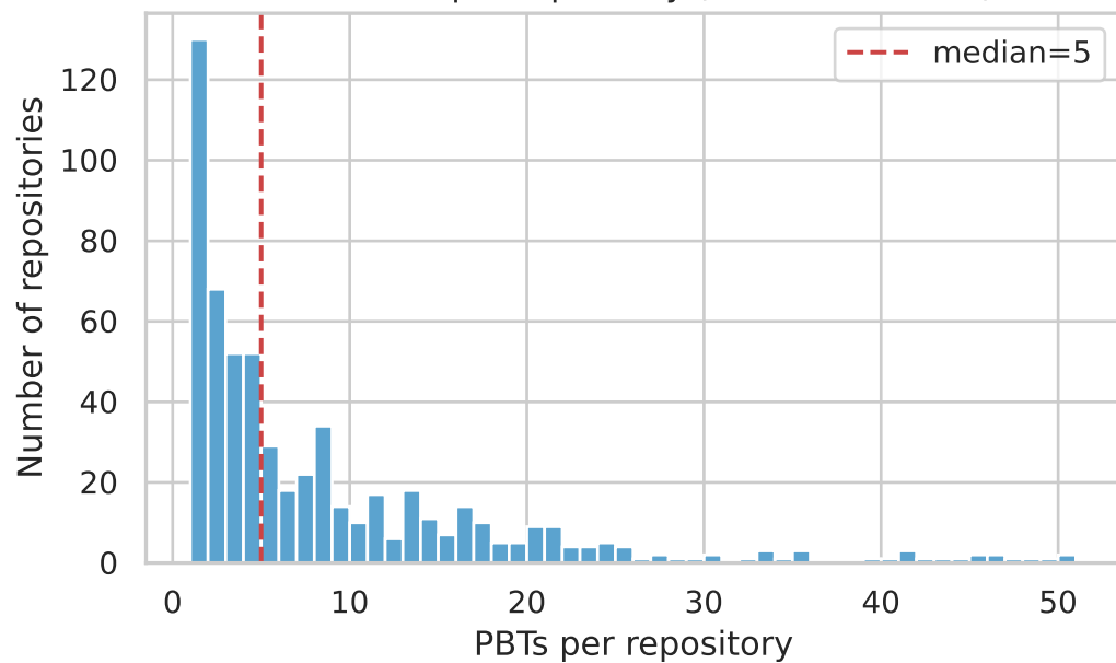
PBT count per repository ( \leq 50 PBTs shown)
