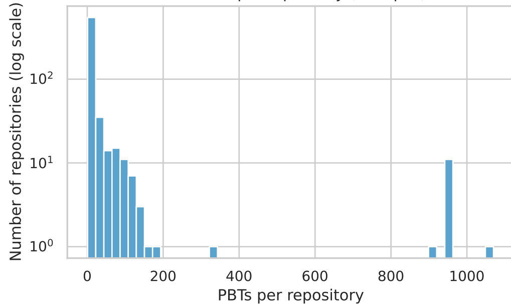
PBT count per repository (all repos)
