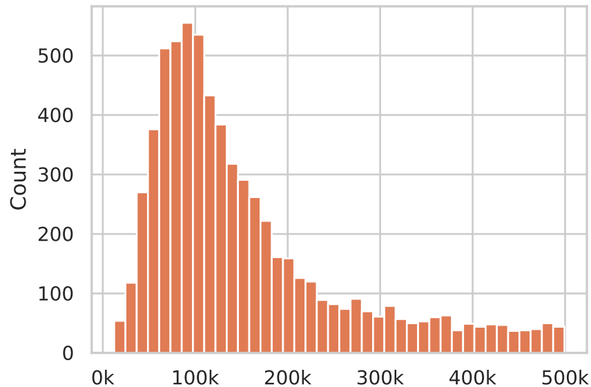
Token cost per sample
