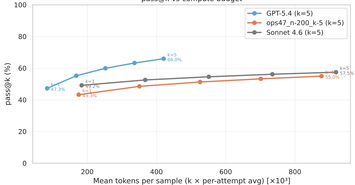
pass@k vs compute budget
