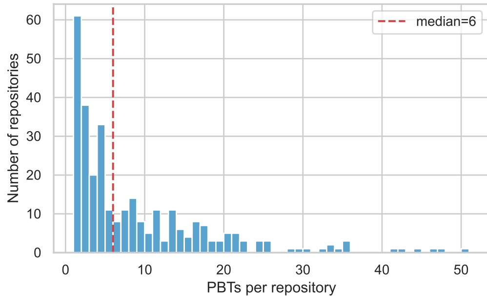
PBT count per repository ( \leq 50 PBTs shown)
