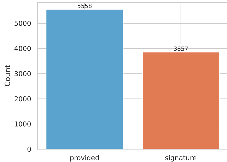
Implementation level
