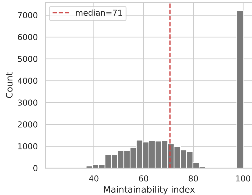
Python maintainability index
