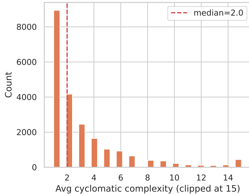
Cyclomatic complexity
