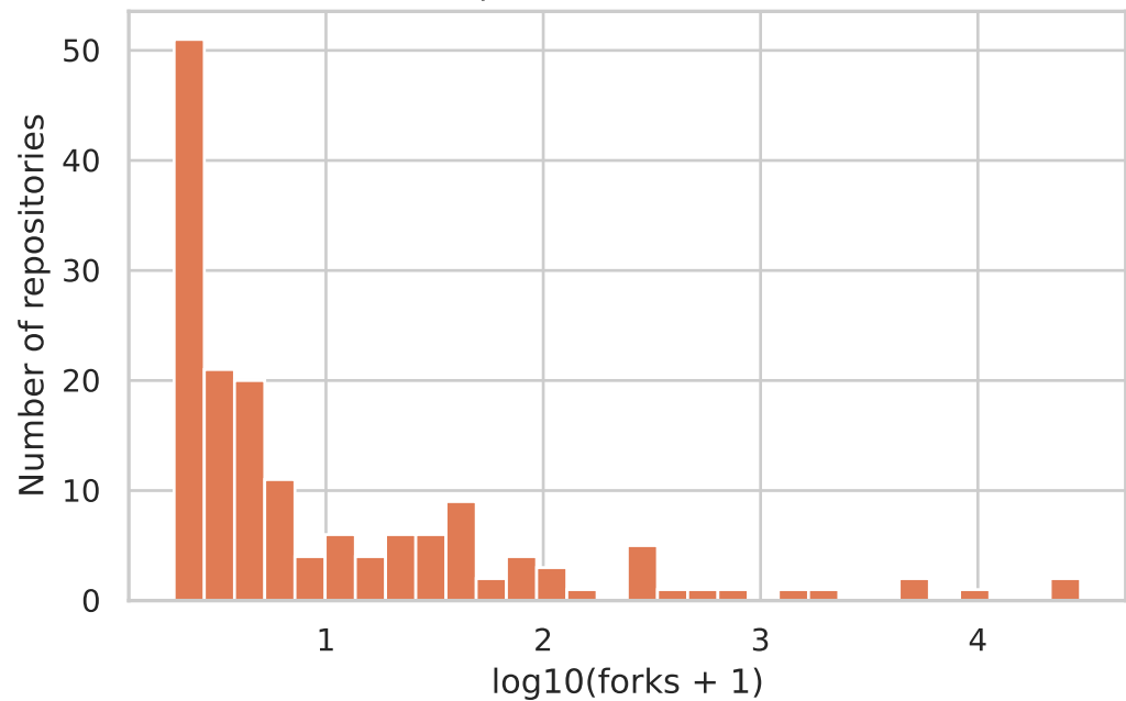
Forks distribution (482 repos with 0 forks omitted)
