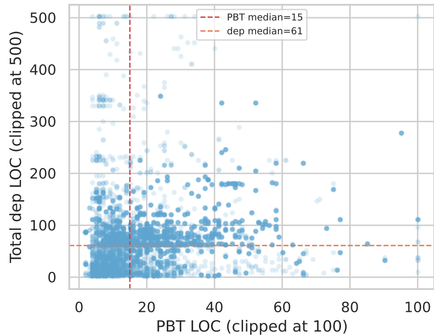
PBT size vs. code under test
