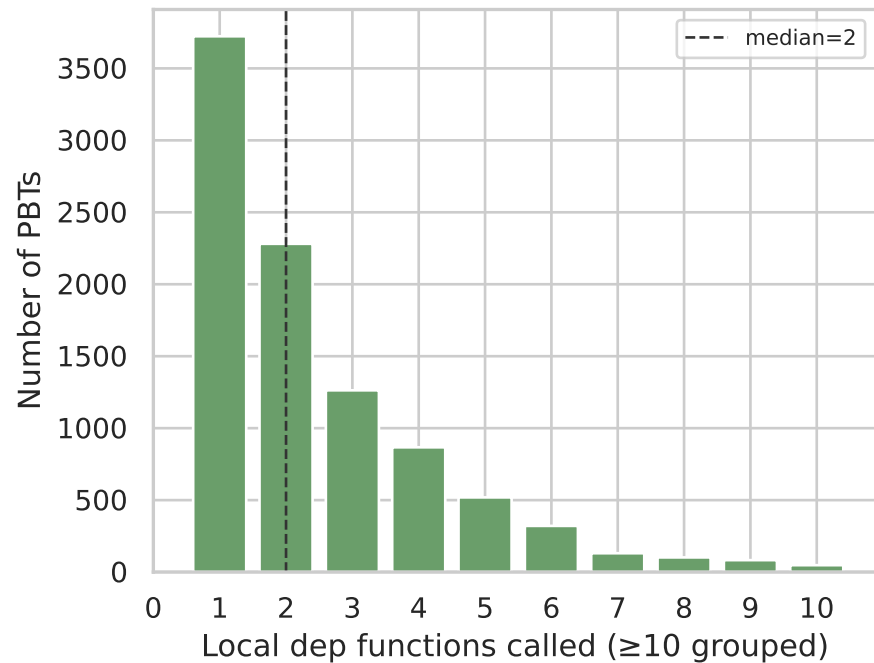
Direct local dependencies per PBT
