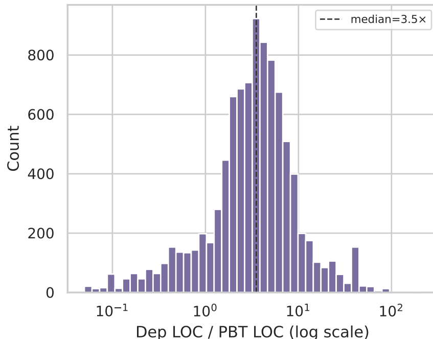
How much larger is the tested code?
