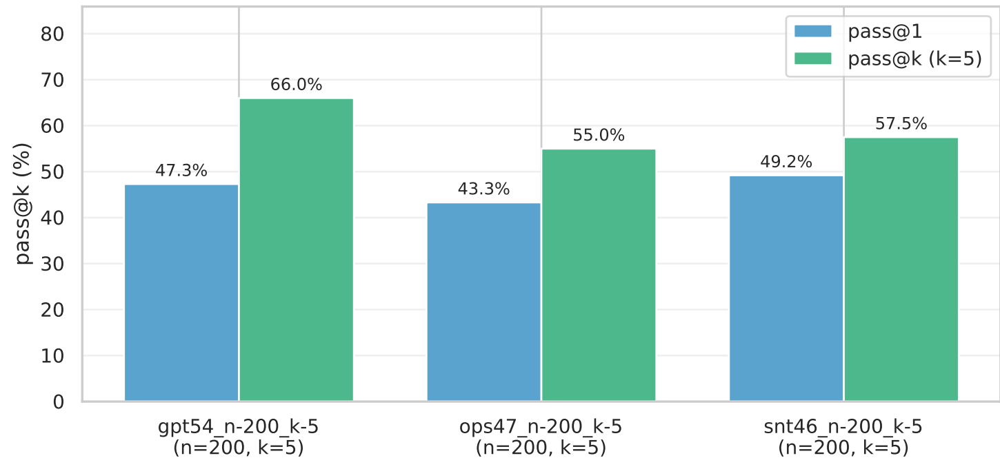
pass@1 vs pass@k
