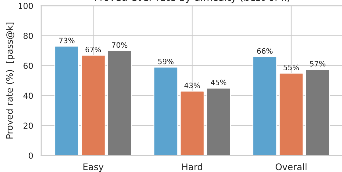
Proved-ever rate by difficulty (best-of-k)
