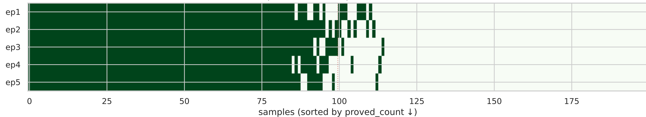
Sonnet 4.6 — proved: 115/200 (pass@5), consistent: 85/200
