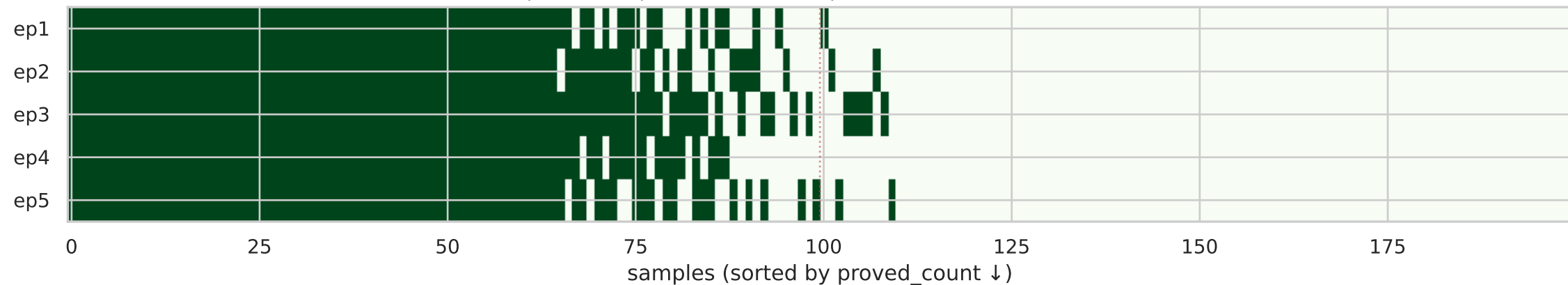
Opus 4.7 — proved: 110/200 (pass@5), consistent: 65/200
