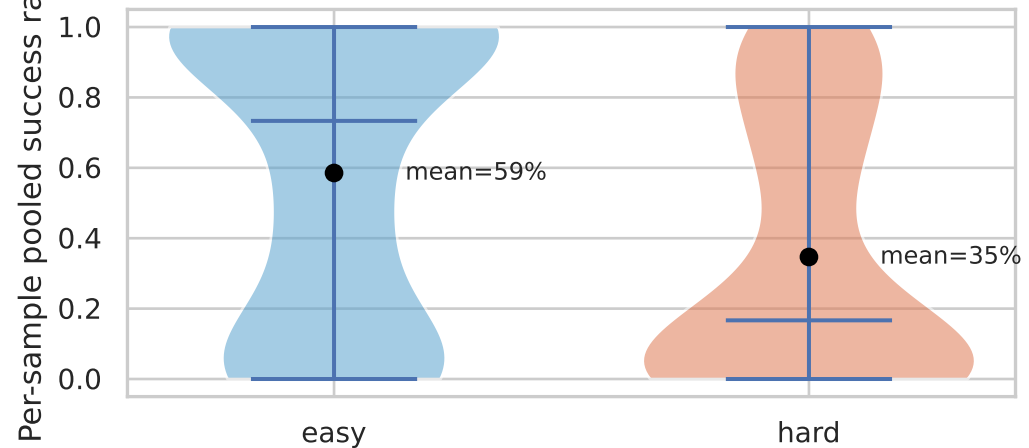
Bucket separation (rank-AUC=0.68)
