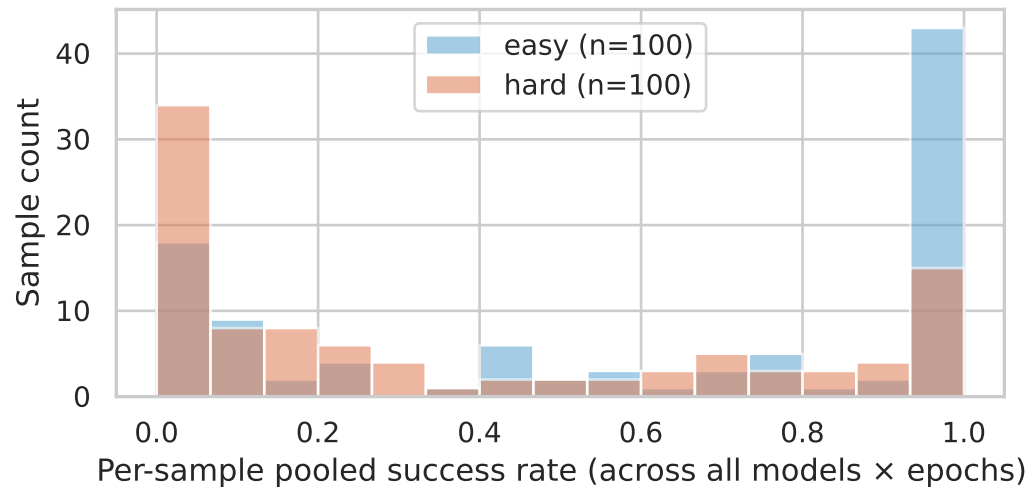
Empirical difficulty distribution by grader label
