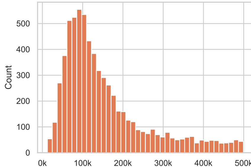
Token cost per sample
