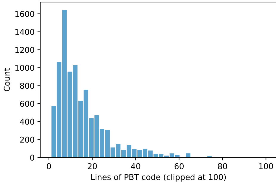
Source PBT size
