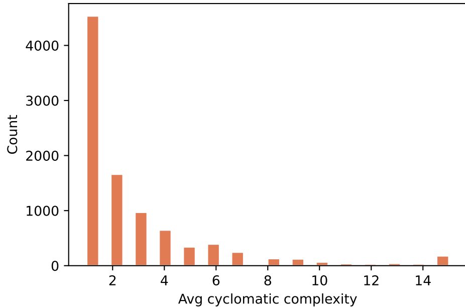
Python source complexity
