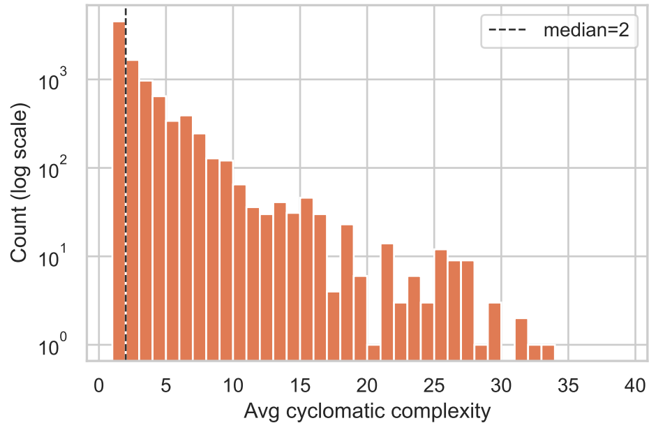
Python source complexity
