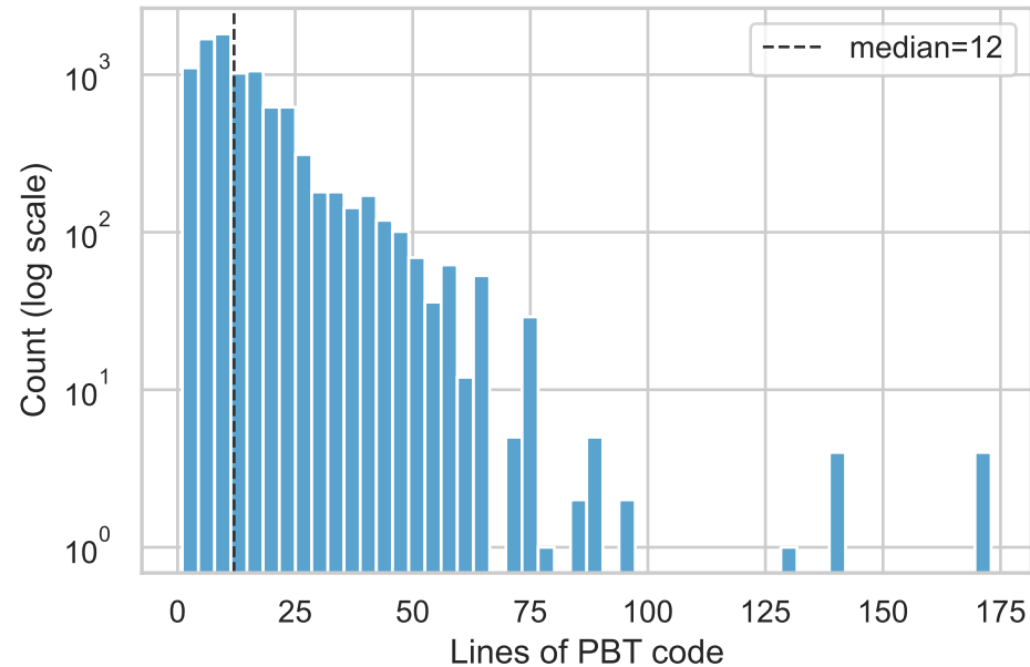
Source PBT size
