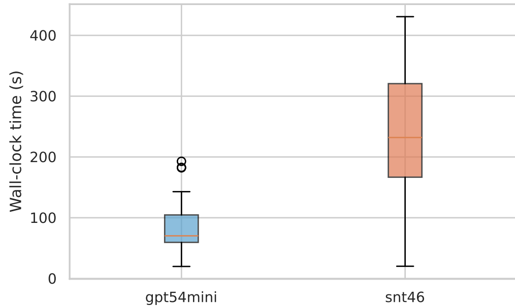
Time per sample
