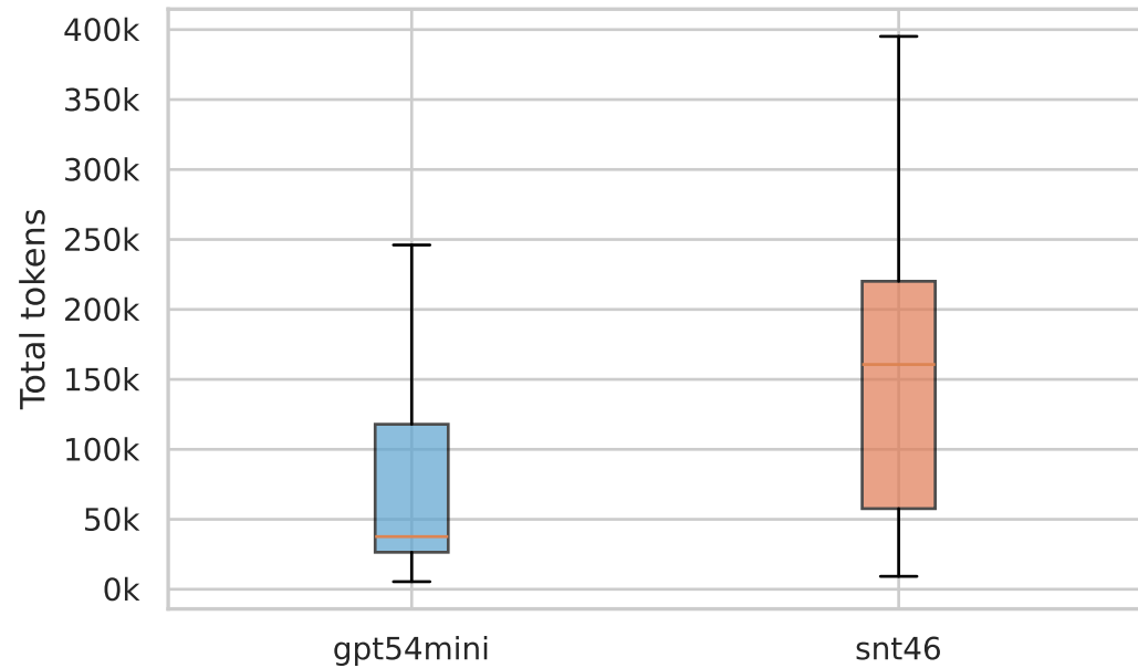
Token usage per sample
