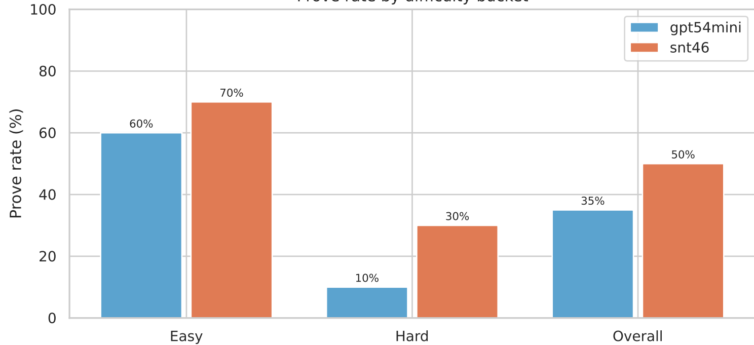
Prove rate by difficulty bucket
