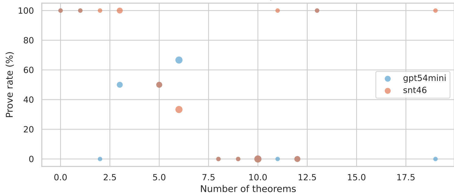
Prove rate vs. theorem count (bubble size = sample count)
