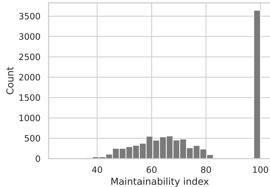
Python maintainability index
