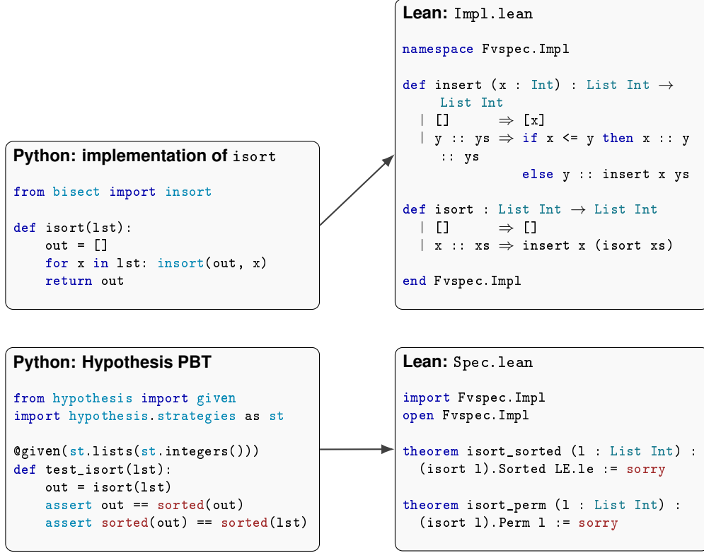
Figure 1: The four artifacts of a single FVSpec problem. Top: the Python implementation of isort and its complete Lean port. Bottom: the Hypothesis PBT and the corresponding Lean theorems. The AI must replace both Lean sorry placeholders—one per theorem.
