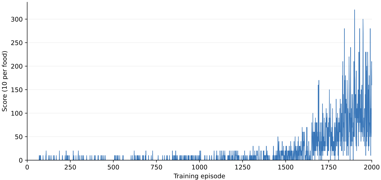
Historical: original DQN training
