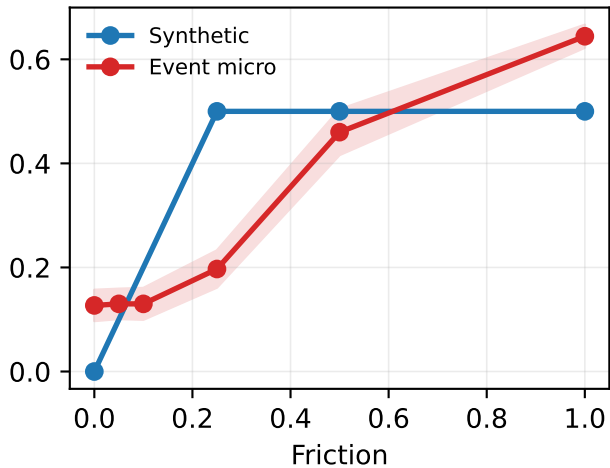
Ranking disagreement with 95% bands
