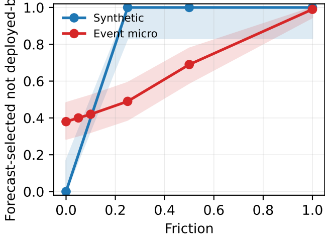
Deployed-suboptimal share with 95% bands
