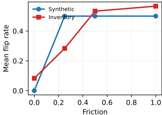
Flip rate
