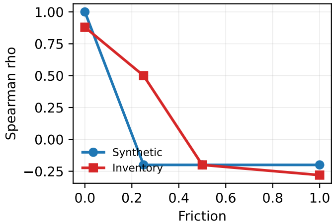
Rank correlation
