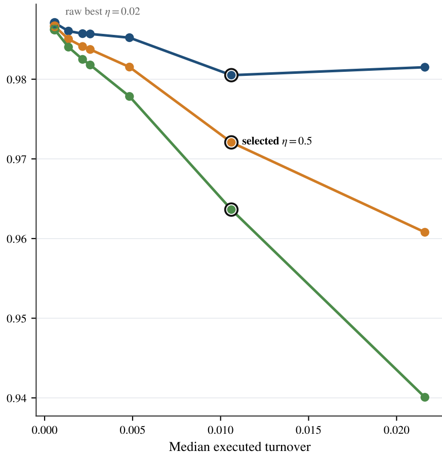
U36 Replication
