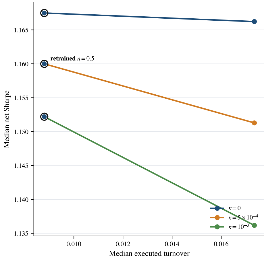
Eta-Aligned Retraining
