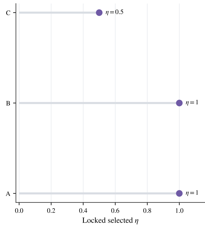
Selected-Point Transfer
