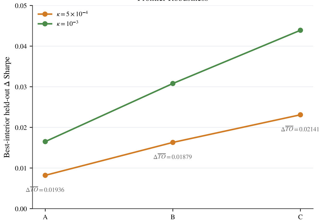
Frontier Robustness
