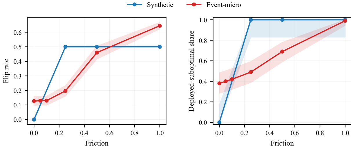
Figure A4. Q2 uncertainty summaries for synthetic and event-micro. Left: flip rate; right: deployed-suboptimal share. Bands follow the interval convention described in Appendix G; zero-width bands may coincide with the line.
