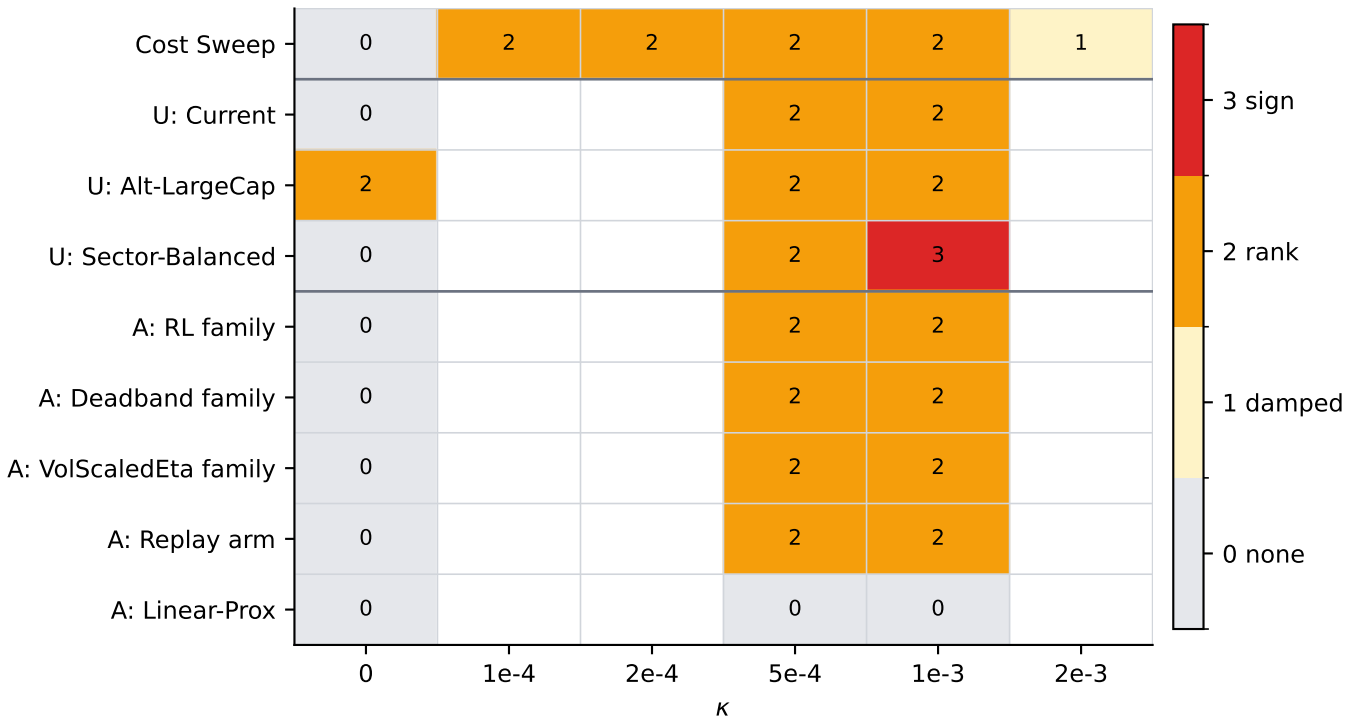
Meta Disagreement Summary Across Support Packages
